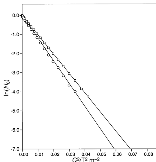
Fig. 2 ^1\text{H} diffusion results for compounds 3 (squares) and 4 (circles) in \text{CDCl}_3 . The slopes are quite different despite identical positive fragments. This is due to the existence of 3 as a tight ion pair and to the presence of the large counter ion \text{BARF} , which almost doubles the molecular volume of 3 .
